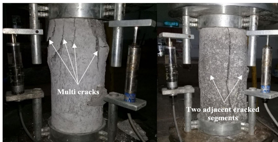
FIGURE 7 | Cracks failure for granite-based geopolymer concrete (G-GPC) and palm oil clinker-based geopolymer concrete (P-GPC) under compression [23]. Reprinted with permission from Elsevier (2022).
