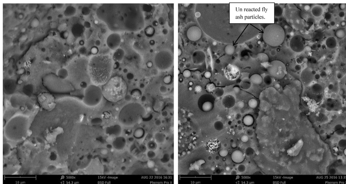
FIGURE 9 | Scanning electron microscopy (SEM) images of (a) control geopolymer concrete (GPC) and (b) GPC with 100% palm oil clinker (POC) aggregate [67]. Reprinted with permission from Elsevier (2021).
