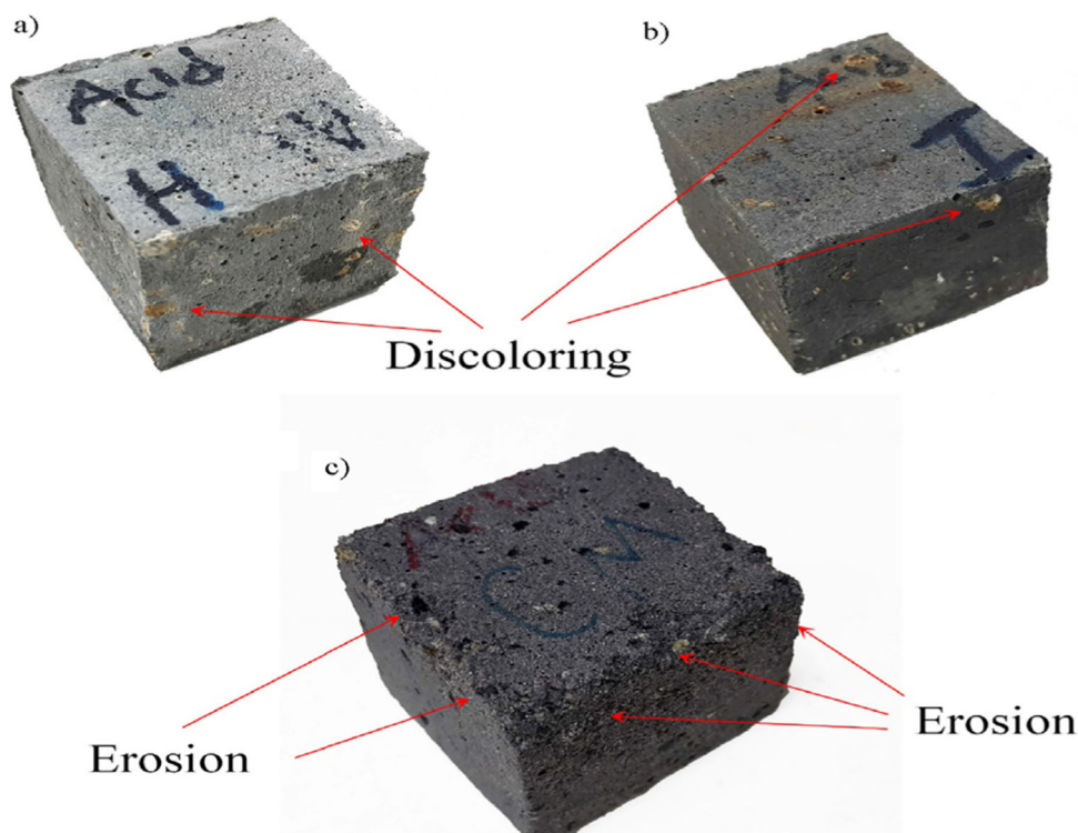
FIGURE 6 | Physical appearance of samples exposed to HCl: (a) FA-MS-based geopolymer mortar (GPM), (b) FA-GGBS-POC-based GPM, and (c) cement-MS mortar [34]. Reprinted with permission from Elsevier (2020).
