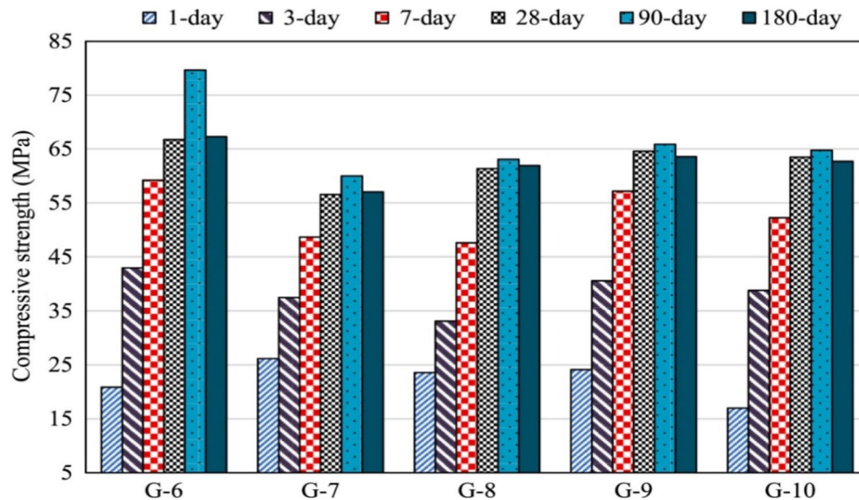
FIGURE 5 | Effect of palm oil clinker (POC) aggregate content on the compressive strength of geopolymer mortar (GPM) [52]. Reprinted with permission from Elsevier (2021).
