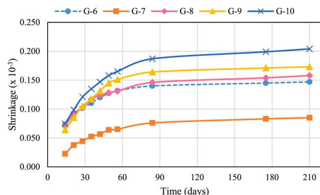
FIGURE 8 | Drying shrinkage of geopolymer mortar (GPM) [52]. Reprinted with permission from Elsevier (2021).
